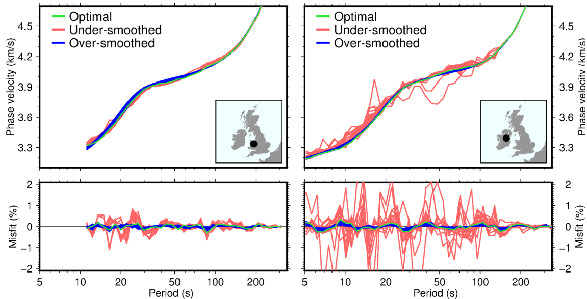
Figure 9. Selection of the optimal inversion smoothing for a point, based on the estimated errors of the phase-velocity curves yielded by phase-velocity maps. Top panel: phase-velocity curves at two points in Wales and in Ireland. The locations are mapped in the insets. The curves are extracted from phase-velocity maps with different levels of smoothness. Bottom panel: the period-dependent error of each phase-velocity curve. The error is estimated as the roughness of the phase-velocity curve, which we isolate by fitting it with a synthetic in a very weakly regularized inversion. Red lines: the curves obtained from rough maps. Blue lines: the curves obtained from smooth maps. Green line: the curve chosen as optimal.
