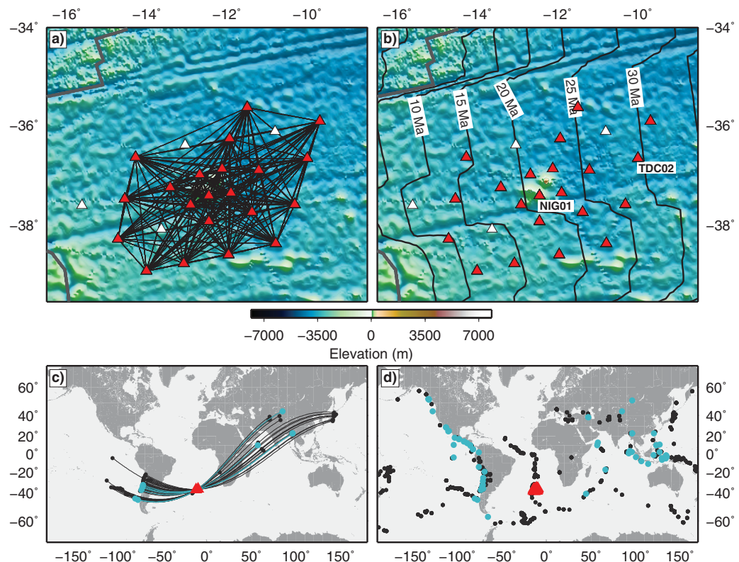
Figure 2. (a) Station locations (triangles) and interstation path coverage (black lines) yielded by our measurements. White triangles are stations with no data available. (b) Seismic stations and the seafloor age. The highlighted stations NIG01 and TDC02 are used in the following to illustrate the measurements (Figures 3 and 4). (c) Distribution of the events used to measure phase-velocity curves with the two-station method for the NIG01-TDC02 station pair; blue dots represent the events producing accepted measurements, out of all the events considered (blue and black). (d) Distribution of the events used to measure phase-velocity curves with the two-station method for all the pairs; blue dots represent the events used for the final set of accepted measurements. Topography and bathymetry are from the GINA (Lindquist et al., 2004) and ETOPO2 (NOAA, 2006) data sets.
